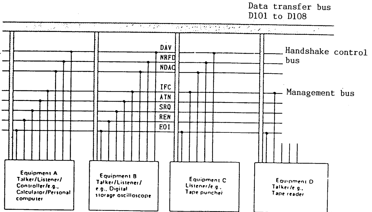
Fig. 10-2 GPIB structure
