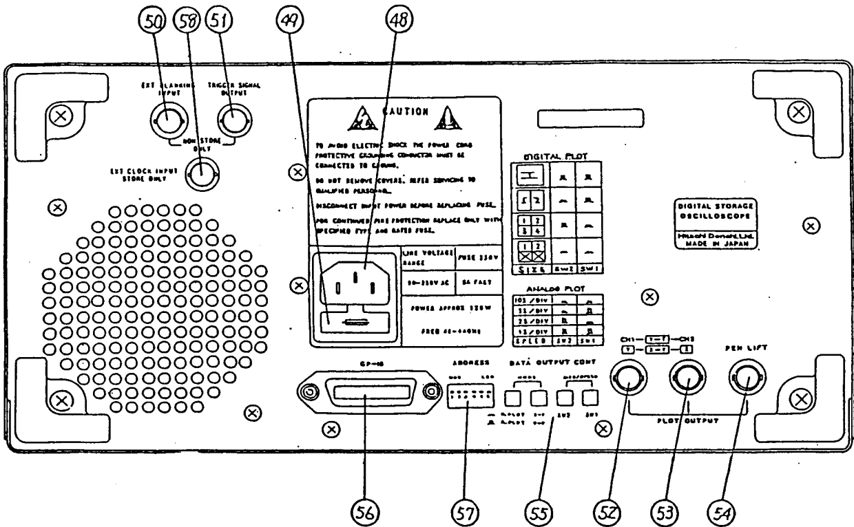
Fig. 5-3 Rear panel
