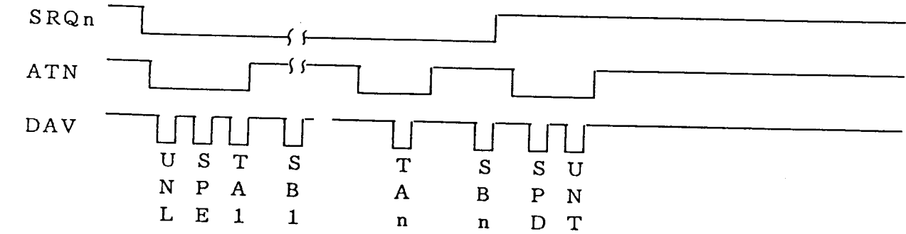
(a) Method most faithful to the IEEE-488 (1975) standards to read status bytes serially.
