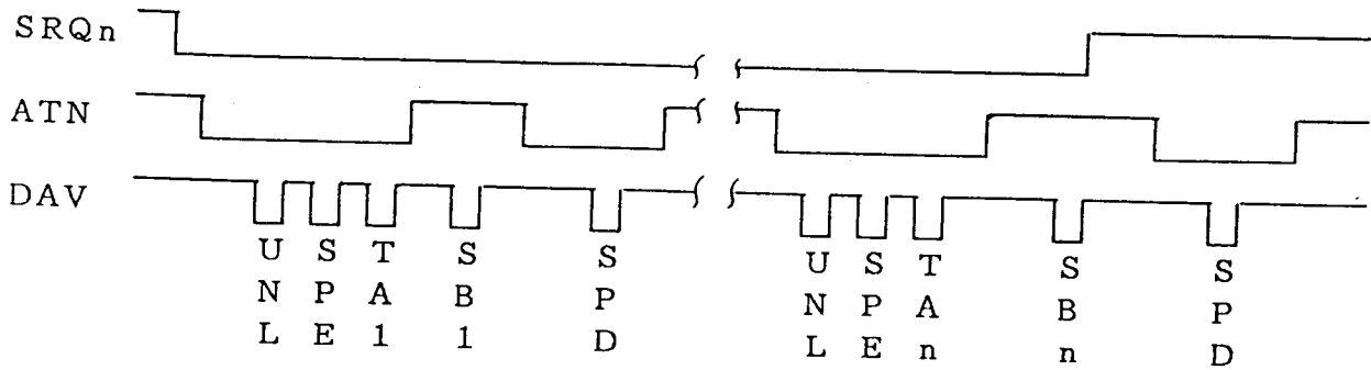
(b) Method to read status bytes one by one (UNT is not inserted after SPD.)
