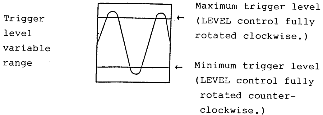
(a) Input signal of large amplitude
