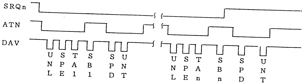
(c) Method to read status bytes one by one (UNT is inserted after SPD.)
