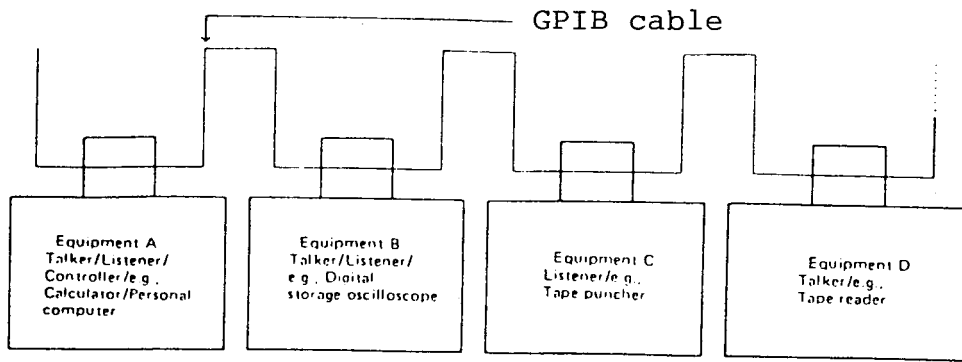
Fig. 10-1 A typical system using the GPIB
