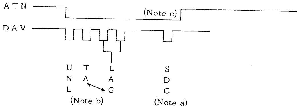
Fig. 10-5 Address command
