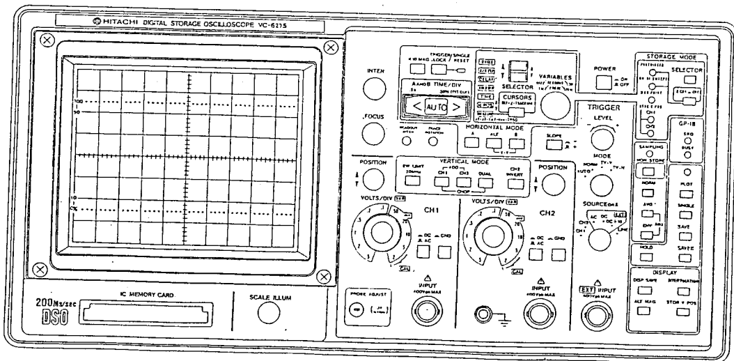
Fig. 4-1 (a) Front View (VC-6275)
